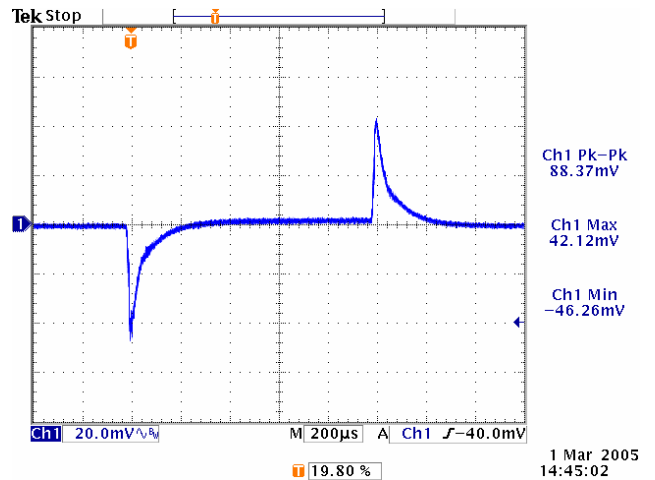
Figure 21. Vin=5V, Vout=1V, BW~60kHz.
