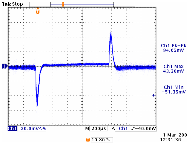
Figure 18. Vin=12V, Vout=5V, BW~60kHz.
