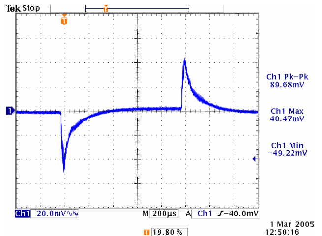
Figure 22. Vin=3.3V, Vout=1V, BW~60kHz.
