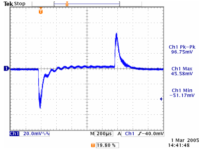
Figure 20. Vin=5V, Vout=2.5V, BW~60kHz.
